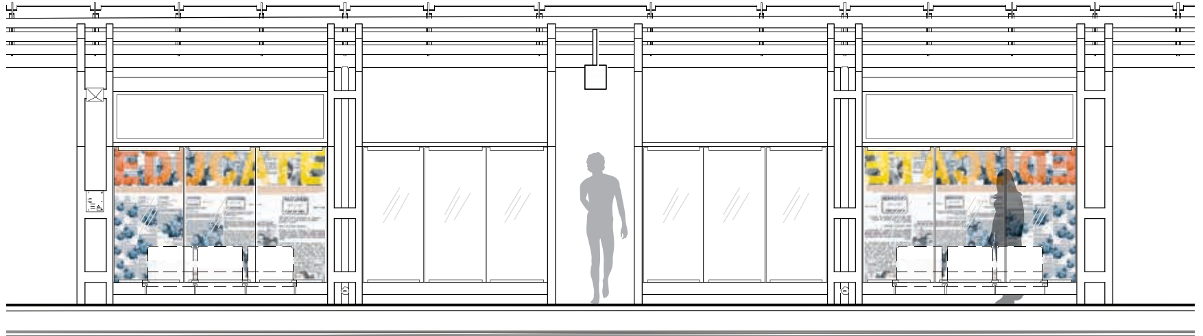
WINDSCREEN PANELS FRONT ELEVATION
